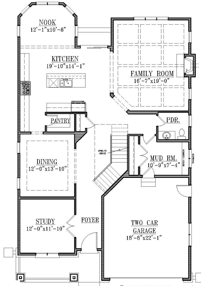
SECOND FLOOR
